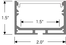
ALP-160 | SURFACE OR SUSPENDED MOUNT
