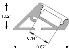
ALP-110 | SURFACE MOUNT
