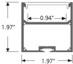
ALP-200 | SURFACE OR SUSPENDED MOUNT
