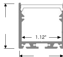
ALP-140 | SURFACE OR SUSPENDED MOUNT
