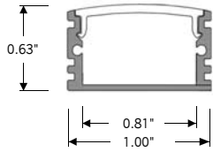
ALU-DS100 | SURFACE MOUNT
