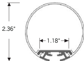
ALP-245 | SUSPENDED MOUNT
