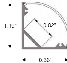
ALP-100C | SURFACE MOUNT
