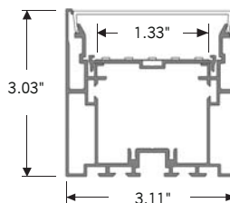
ALP-310N | SURFACE OR SUSPENDED MOUNT
