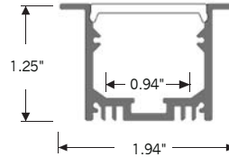
ALP-200R | RECESSED MOUNT
