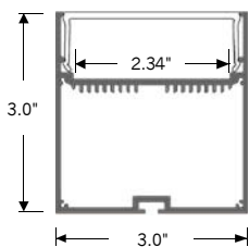
ALP-300 | SURFACE OR SUSPENDED MOUNT
