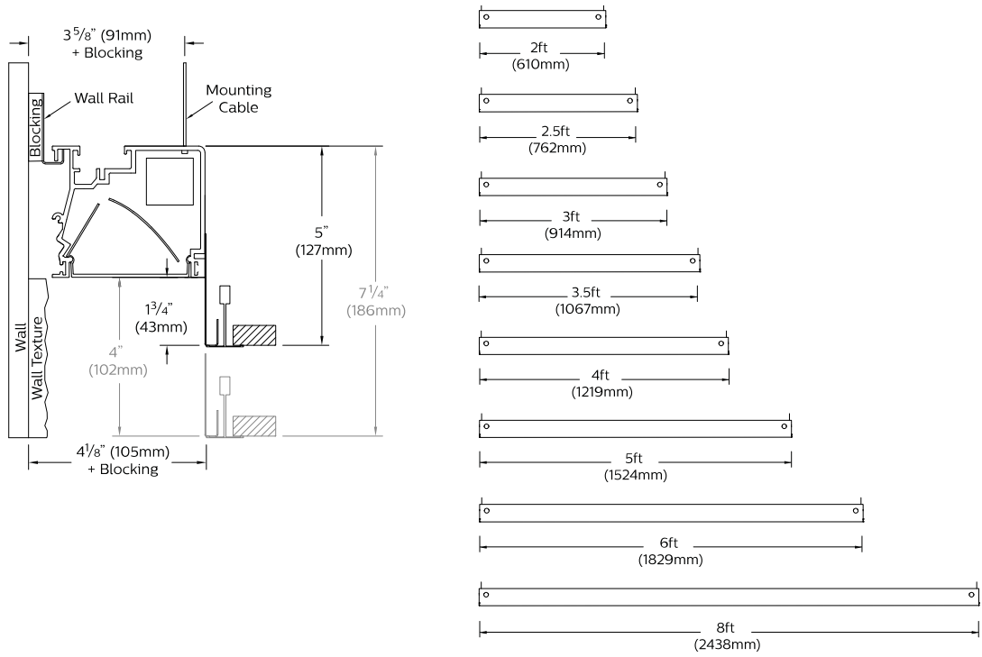
Side View
