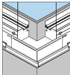
Outside Corner
