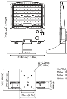
100W/140W/180W (Wall Mount)
