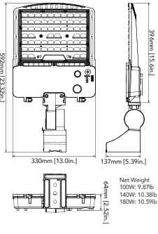
100W/140W/180W (Adjustable Square Mount)
