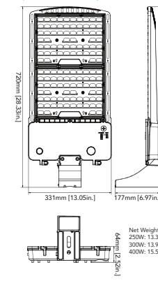
300W/400W (Pole Mount)
