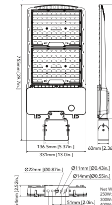
300W/400W (Yoke Mount)
