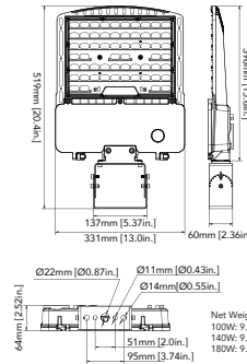
100W/140W/180W (Yoke Mount)
