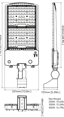
300W/400W (Adjustable Square Mount)
