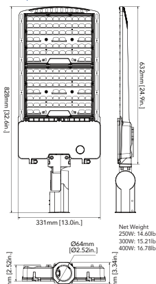
300W/400W (Slipfitter Mount)
