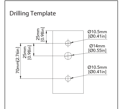
100W/140W/180W (Yoke Mount)
