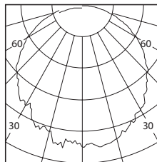
24" LED LIGHT 15300-500
