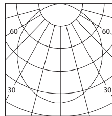
12" LED LIGHT 15300-499
