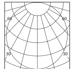
4" LED LIGHT 15300-498
