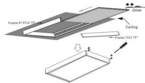
Surface Mounting Frame Kit
